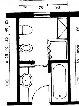
⑰ Bath and shower separated
